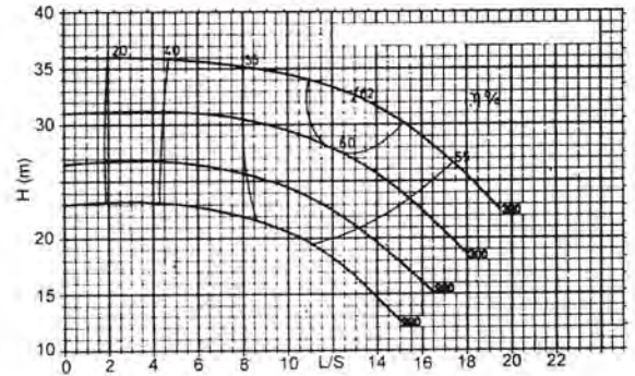
65-32 4poles
