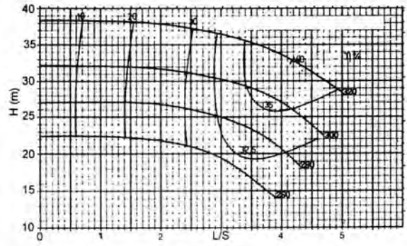
50-32 4poles
