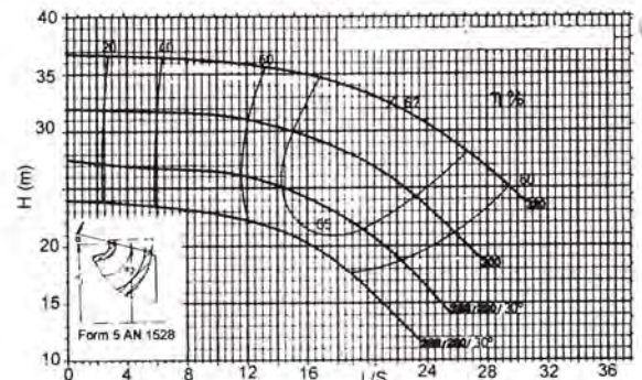
80-32 4poles
