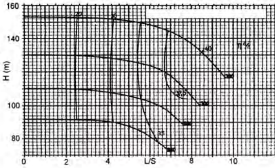
40-32 2 poles
